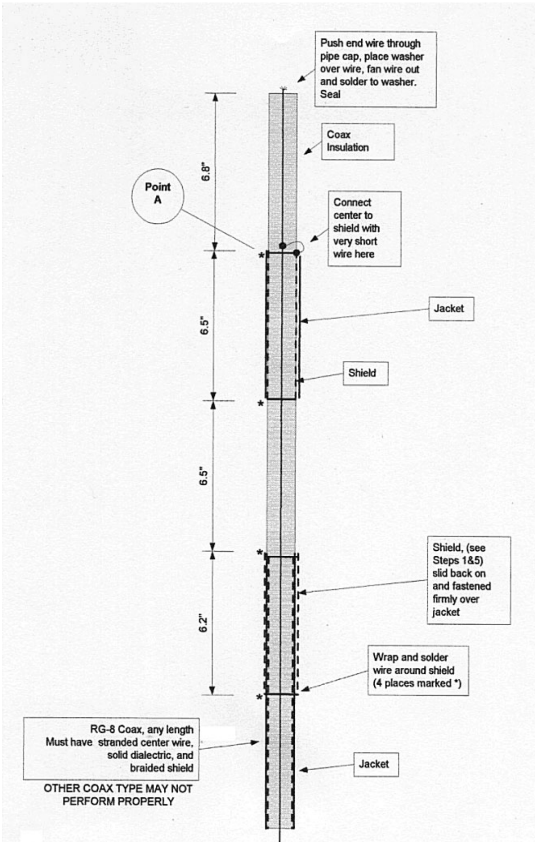
444 MHz Antenna Made from coaxial cable
